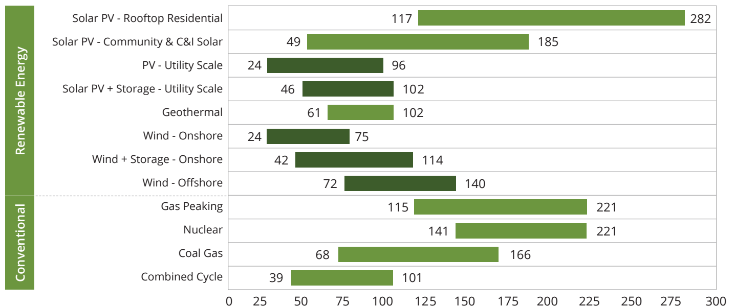
Figure 1. Levelized Cost of Power by Energy Source $/MWh
